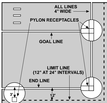
END ZONE DETAIL
